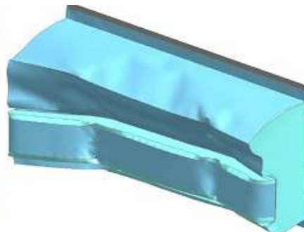
c) Rear-Armature test
