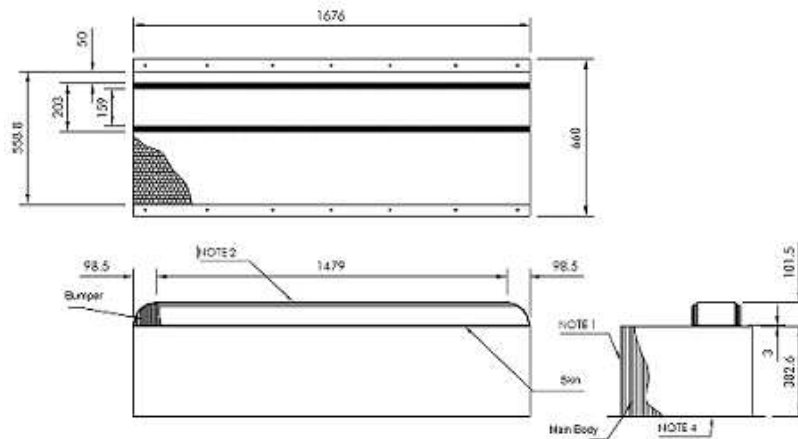
Figure 1. NHTSA Barrier Parts and General Dimensions
