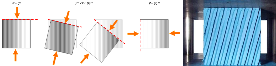
Figure 2. Static angled compressive test procedure
