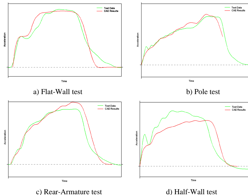
Plot 4. NHTSA model evaluation test results vs. CAE
