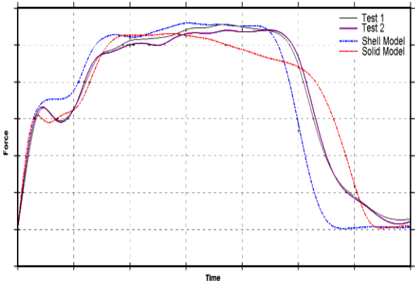
a) Flat-Wall test
