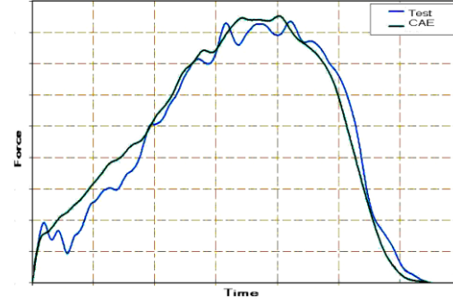
b) AE-MDB Offset Pole test and CAE
