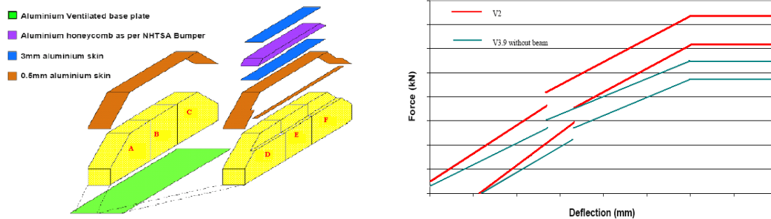
Figure 1. AE-MBD V3.9 parts and a comparison of V2 and V3.9 barrier strength corridors
