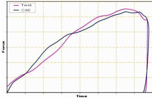
Figure 6. AE-MDB Load-Cell test and FE model
