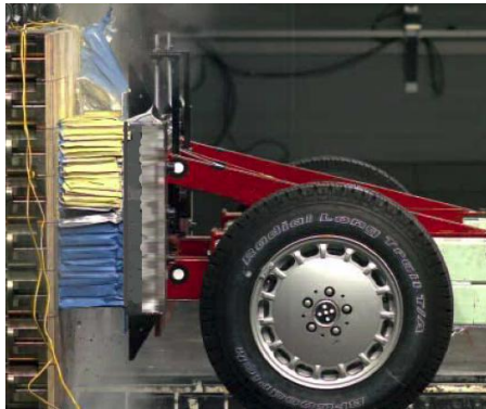
Figure 6. AE-MDB Load-Cell test and FE model
