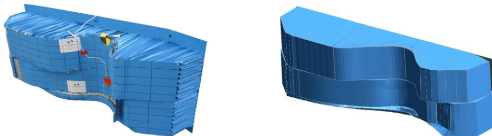
Figure 7. AE-MDB Offset Pole test and FE model
