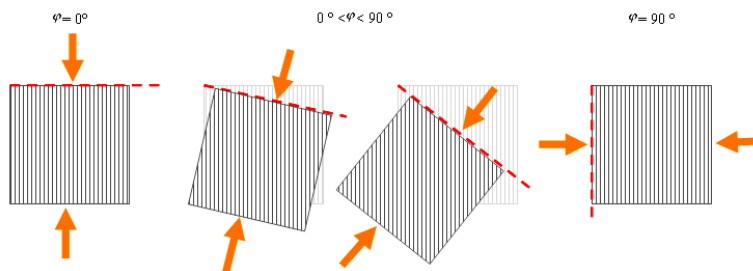
Figure 3. Static angled compressive test procedure
