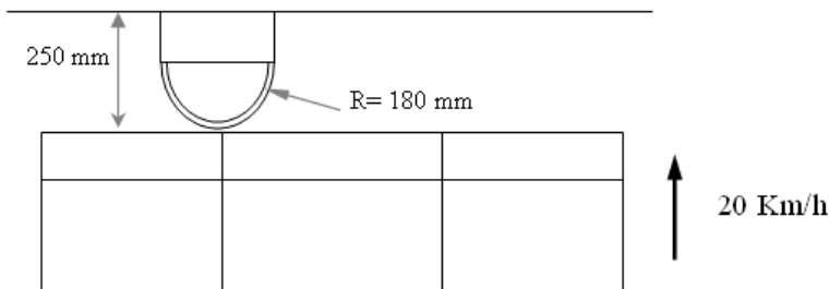
Figure 5. Offset Pole test setup
